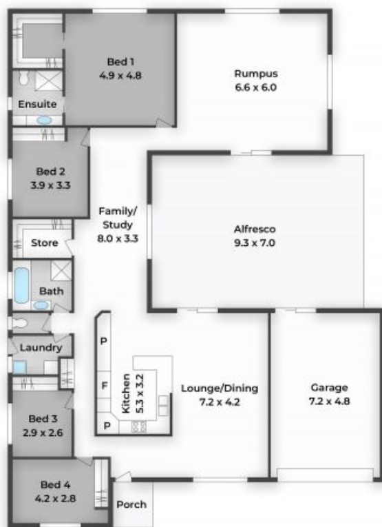
Floor Plan
