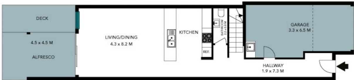
Ground Floor
