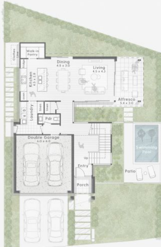
Ground Floor 2.7m Ceiling
