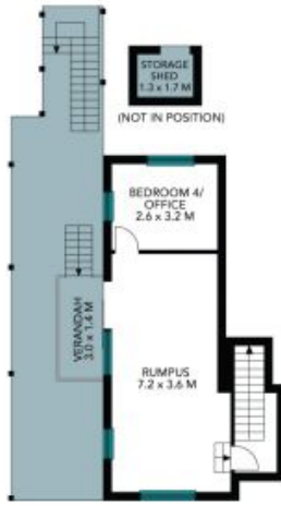
Bottom Floor
