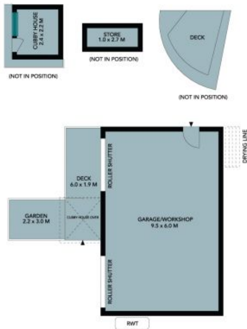
Site Plan
