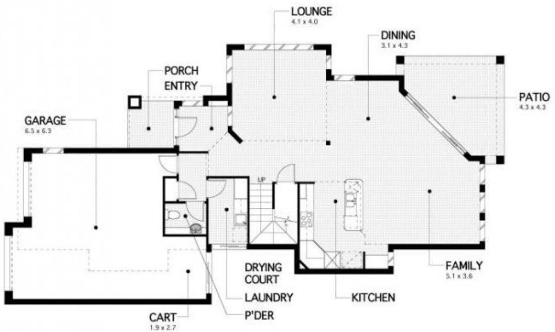
GROUNDFLOORPLAN
